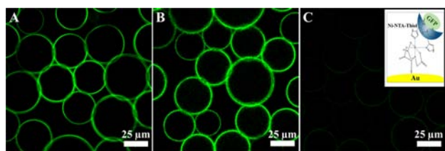
Figure 3. Representative fluorescence images of the GFP-linked gold-nanostructured droplets, measured (A) 1 day, (B) 4 days, and (C) 10 days after their creation. All of the images have the same intensity scale. The right inset schematically shows the chemical immobilization of His6-GFP on a gold NP by means of the Ni-NTA-thiol linker (not to scale).
